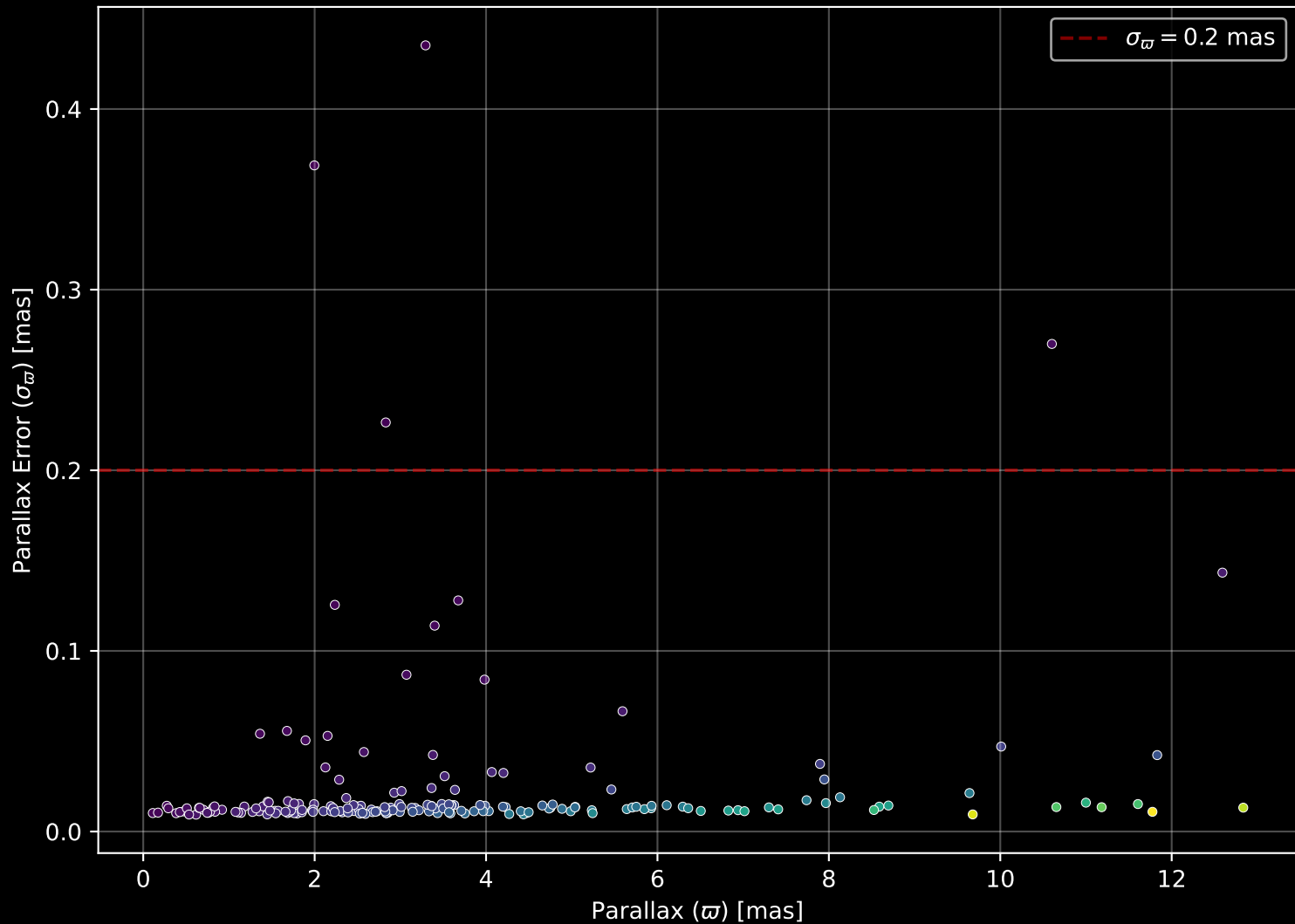
APOGEE DR17 Field: [122+61_MGA] Parallax Quality (n= 193)
