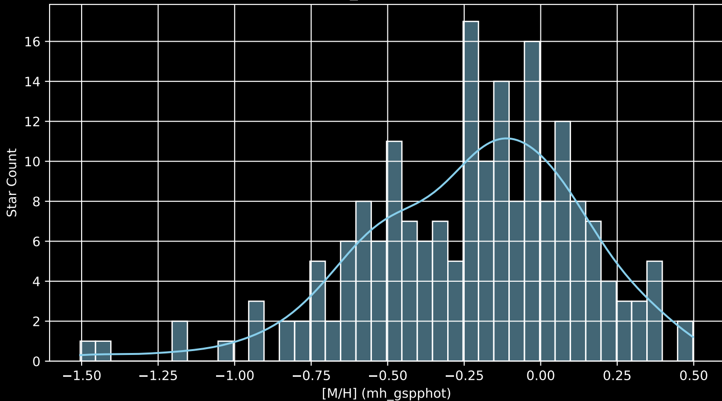
APOGEE DR17 Field: [122+61_MGA [M/H] (mh_gspphot) (n= 192)
