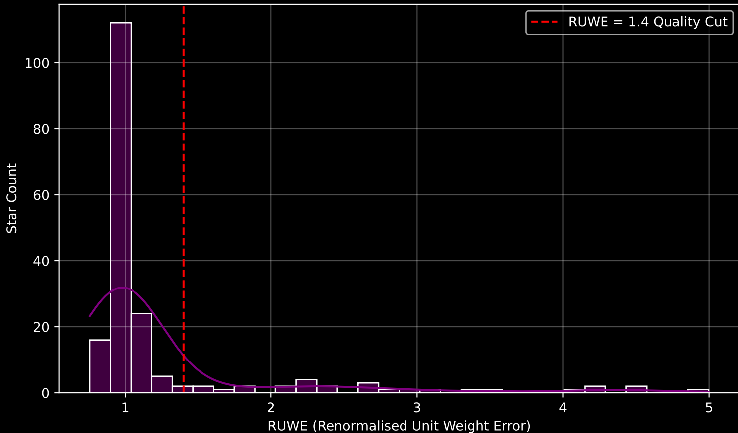
GAPOGEE DR17 Field [122+61_MGA] RUWE Distribution (n= 186)
