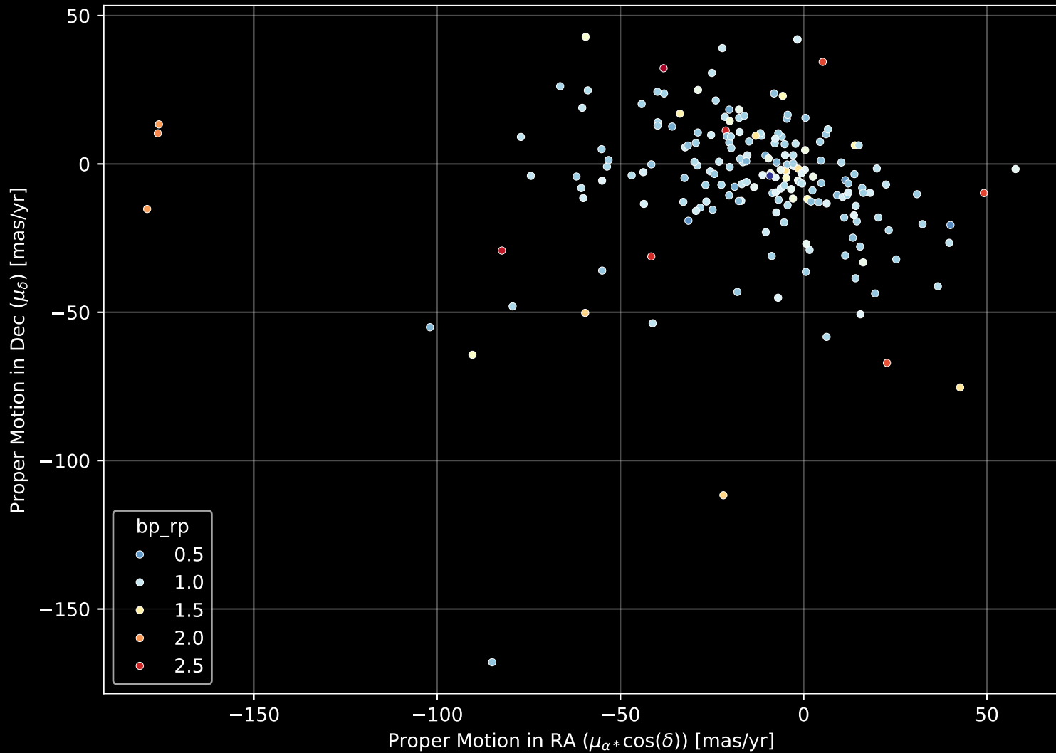
APOGEE DR17 Field: [122+61_MGA] Proper Motion Diagram (n= 193)
