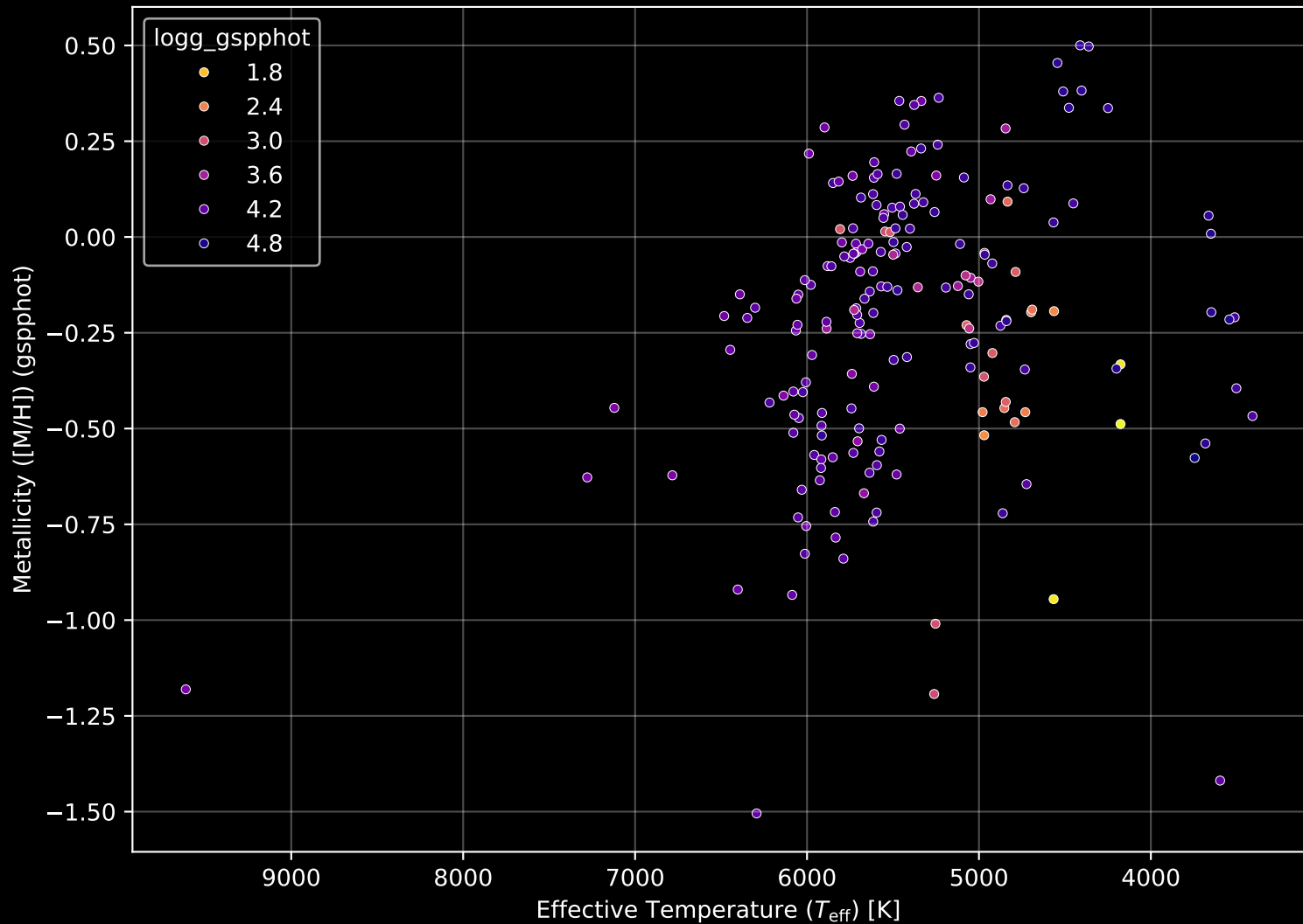
APOGEE DR17 Field: [122+61_MGA] Stellar Population Parameters (n= 193)
