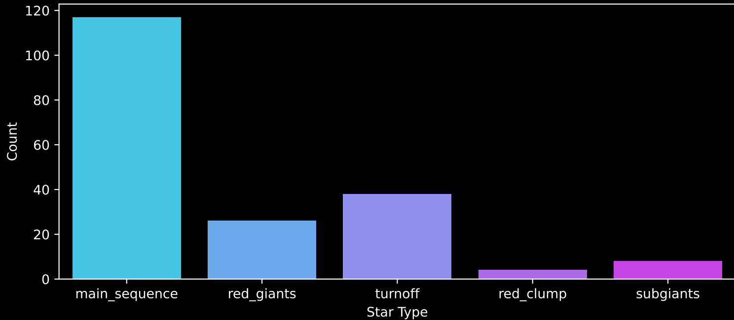
APOGEE DR17 Field: [122+61_MGA] Count plot of Star Type
